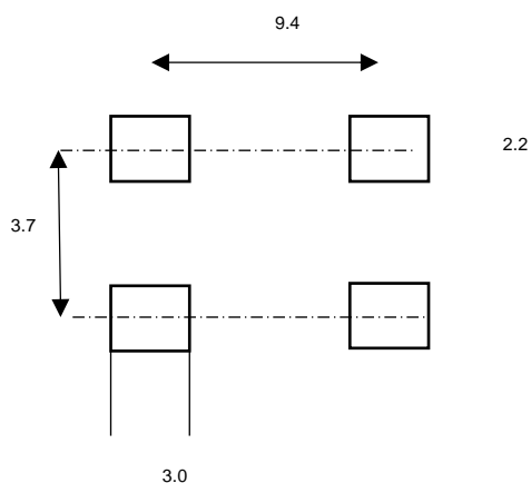
The 86SMX(LPN) series Pad Footprint
