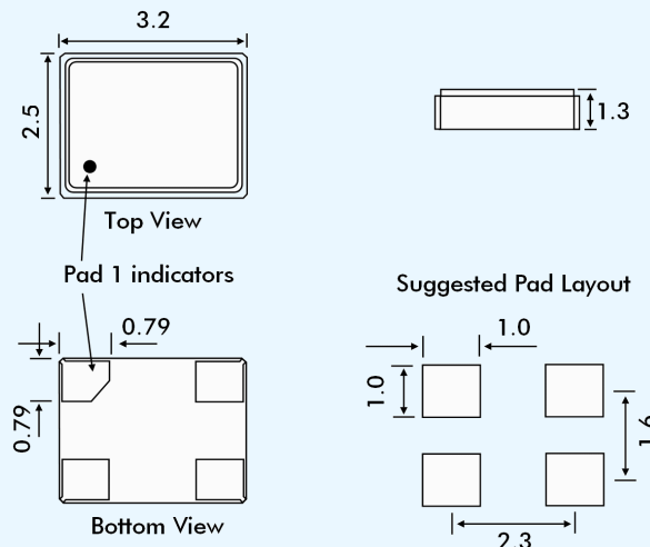
Pad Connections
